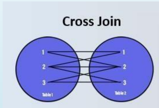
Ven Diagram
